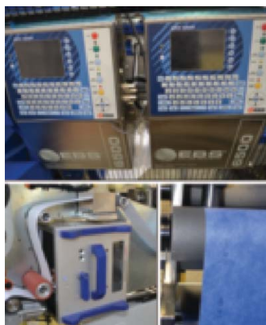
Wide choice of printing options on labels, roll closure tape or direct onto the web
